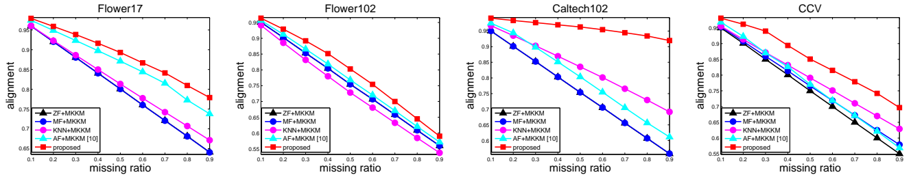
Figure 2: Kernel alignment between the original kernels and the imputed kernels by different imputation algorithms under different missing ratios.
