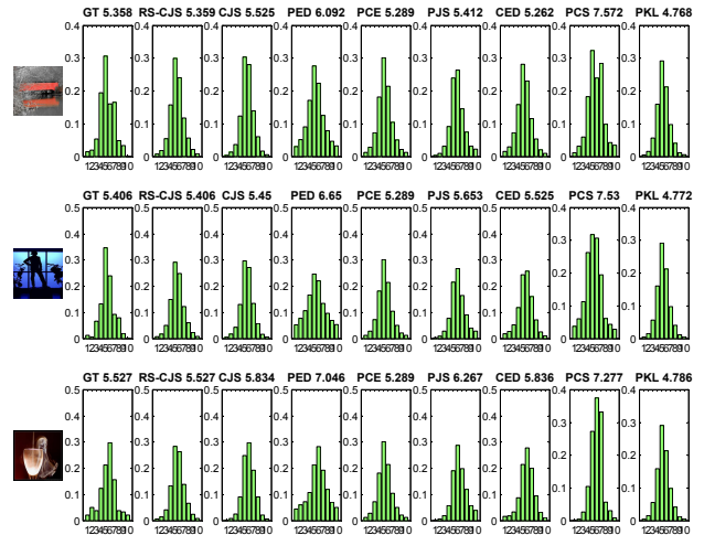
Figure 5: Predicted score histograms by the above loss functions. The numbers above each histograms are their mean scores. The first column is the images. The 2nd column is the human rating distributions (GT: Ground Truth). The 3rd and the 4th columns are the results predicted by our proposed RS-CJS and CJS based CNN, respectively. The other columns are the predicted results of other loss functions. Our results are more similar to the ground truth of human ratings than others. Images are from the AVA dataset (Murray, Marchesotti, and Perronnin 2012), which contains a list of photo IDs from www.dpchallenge.com.
